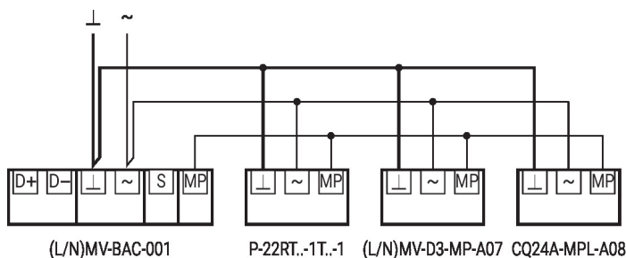
System connection via MP-Bus client-server connections
